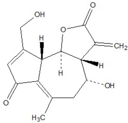
Lactucin
